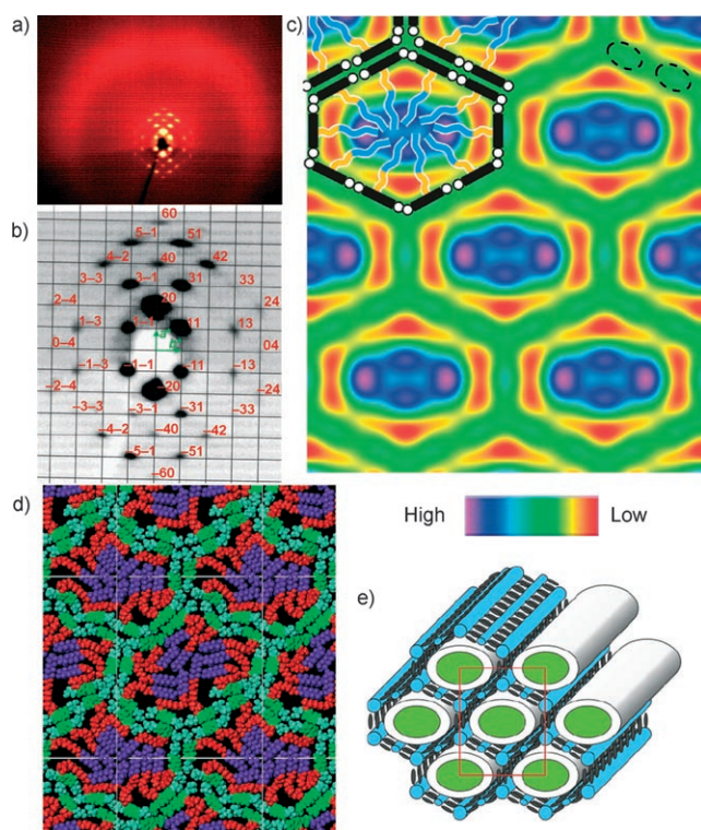
Figure 2. The Col rec /c2mm phase of compound 1 : a,b) X-ray diffraction pattern of a surface-aligned sample at 60 °C; the domains are rotationally disordered around the vertical axis perpendicular to the surface and the X-ray beam; c) reconstructed electron-density map obtained from the small-angle diffraction intensities of a powder pattern (color scale at the bottom); dotted ellipses at the right top indicate the position of the aromatic cores in the elongated cylinder sides which have a slightly increased electron density; the organization of the molecules is indicated at the left top; d) snapshot of molecular dynamics simulation; colors: blue/purple = perfluorinated end groups ( R_F ), green = biphenyl, turquoise = diol groups, red = aliphatic chains (for details, see the Supporting Information); e) sketch of the organization of the molecules in the mesophase.
